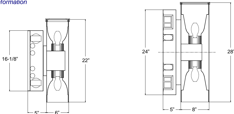
Electronic metal halide ballast option. Suffix catalog number with "E". Metal halide 8" dia. only.
