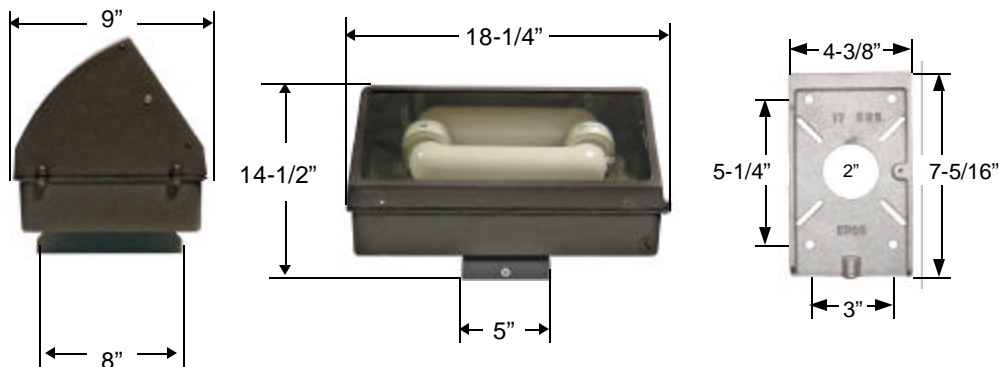
STEP 2. Attach cast aluminum mounting plate on recessed j-box.
